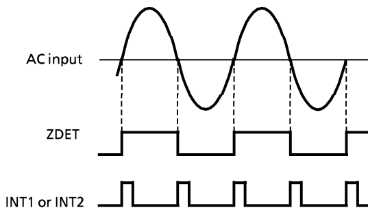
Figure 3-20. Detection Signal
