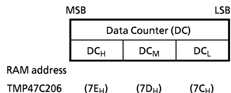
Figure 2-7. Data Counter
