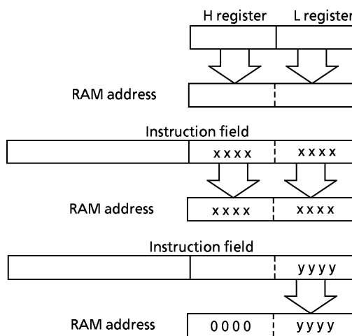
Figure 2-5. Addressing mode
