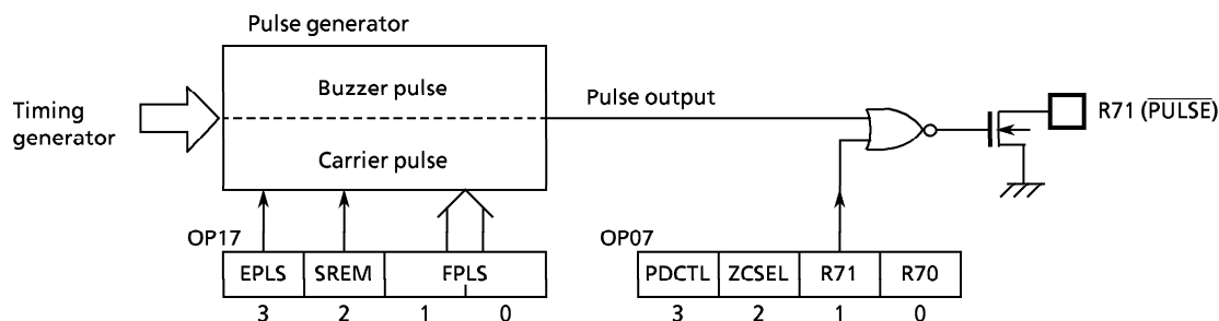
Figure 3-15. Pulse Generator
