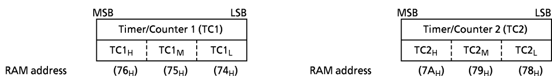
Figure 3-7. The Count registers of the Timer/Counters (TC1, TC2)
