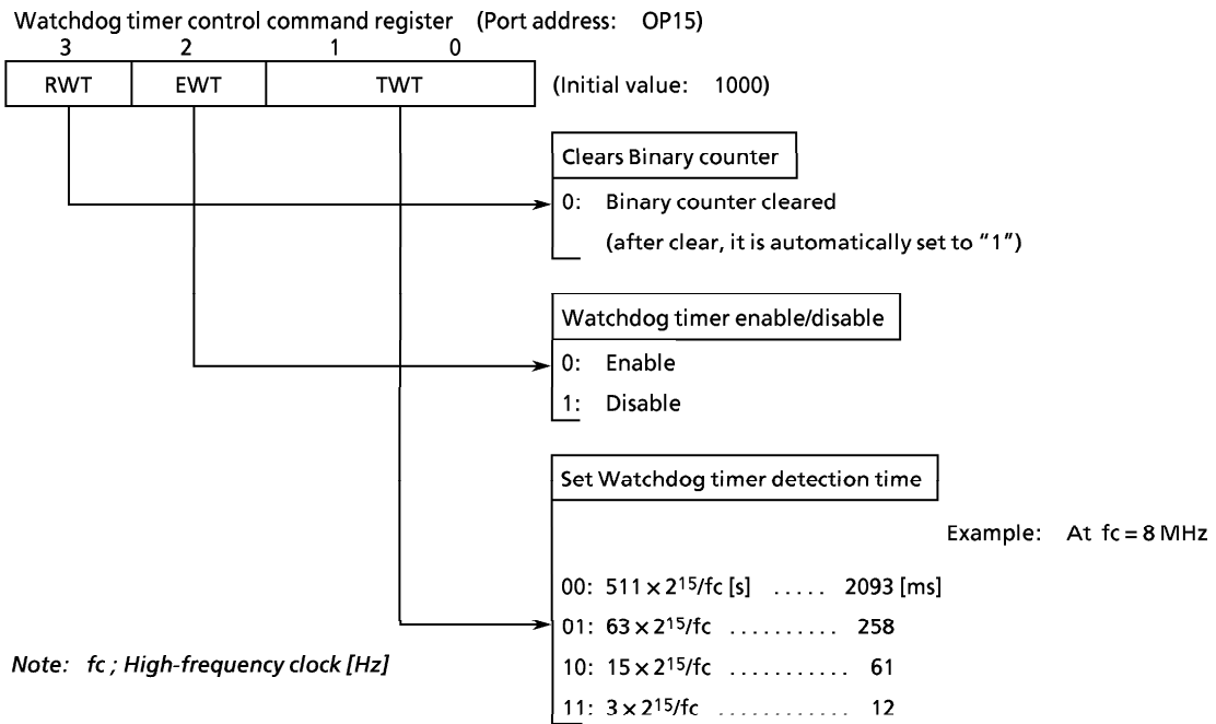
Figure 3-14. Watchdog Timer Control Command Register
