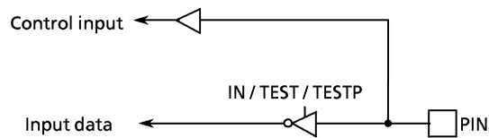
Figure 3-5. Port KE
