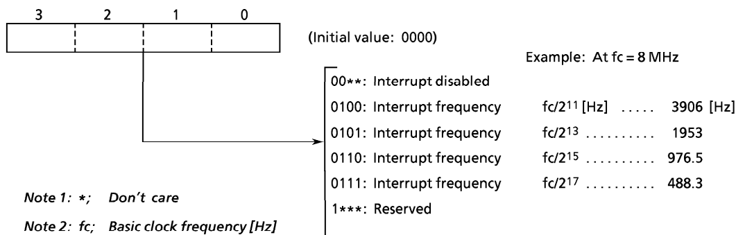
Figure 3-6. Interval Timer Interrupt Command Register
